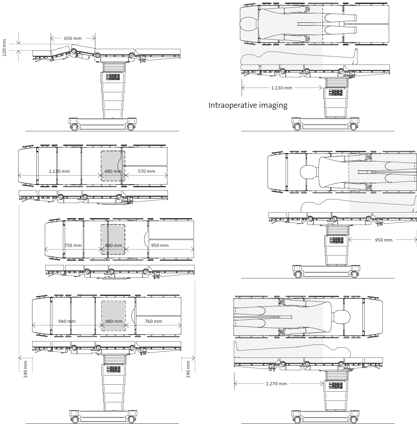
Longitudinal sliding of table top (optional)
